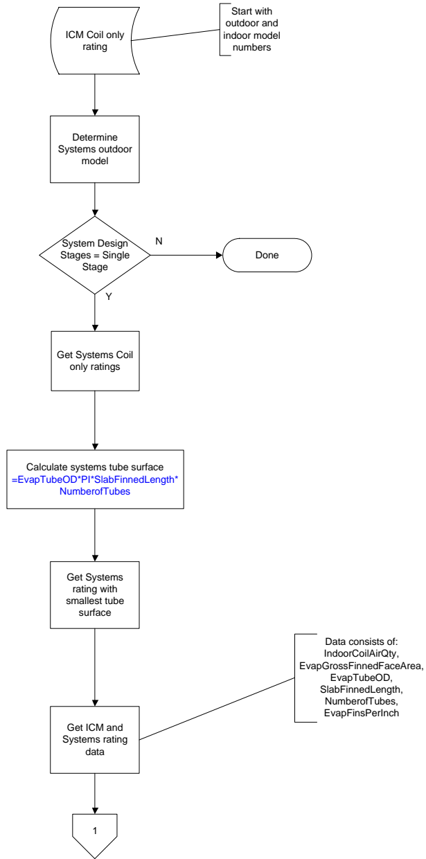
Figure G1: Part 1 of the ORNL Flowchart
