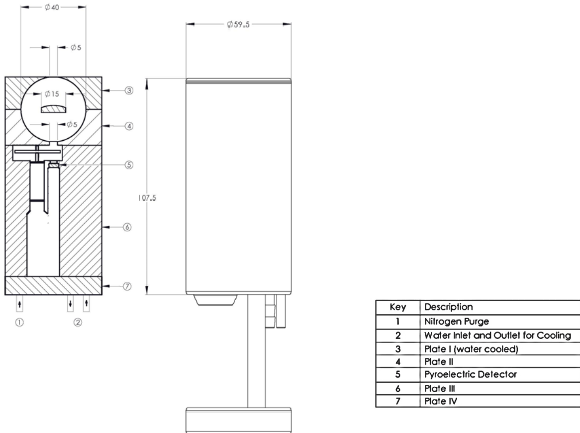
Figure E1. Radiometer Design
