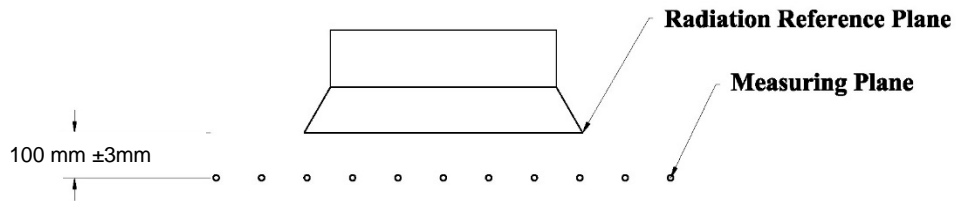
Figure C1. Radiation Reference Plane and Measuring Plane of a Horizontally Mounted High Intensity Infrared Heater
