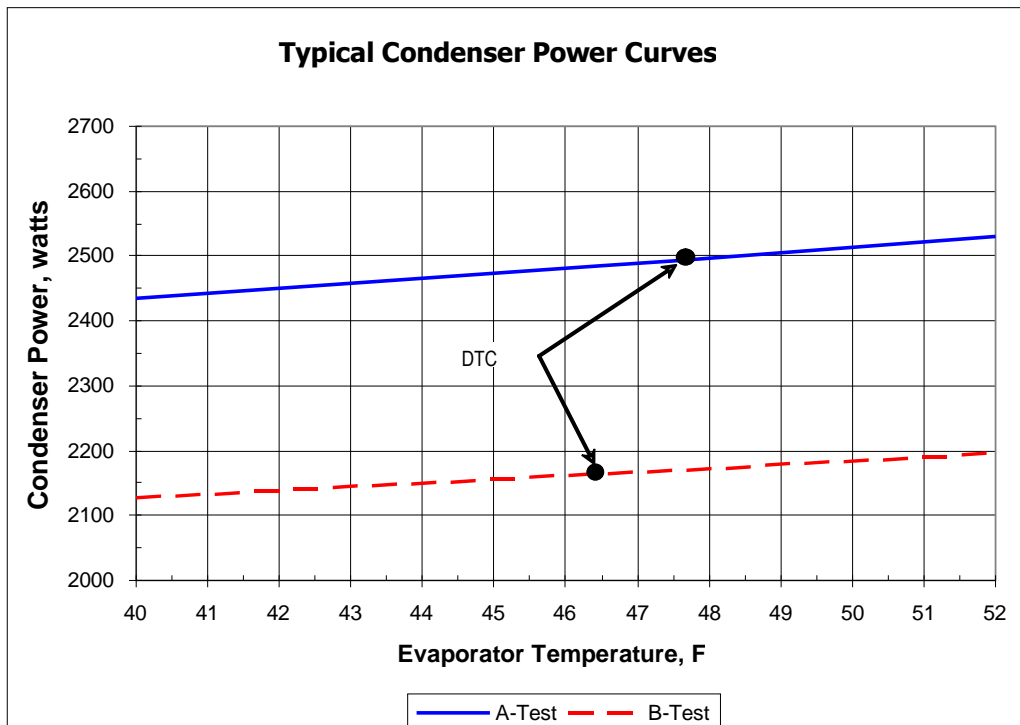
Figure B3: Typical Condenser Power Curves
