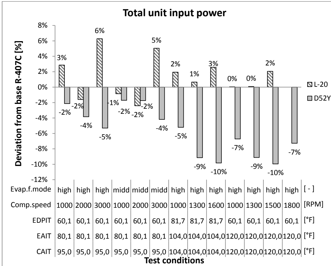
Figure 4: Comparison of total unit input power relative to R-407C.
