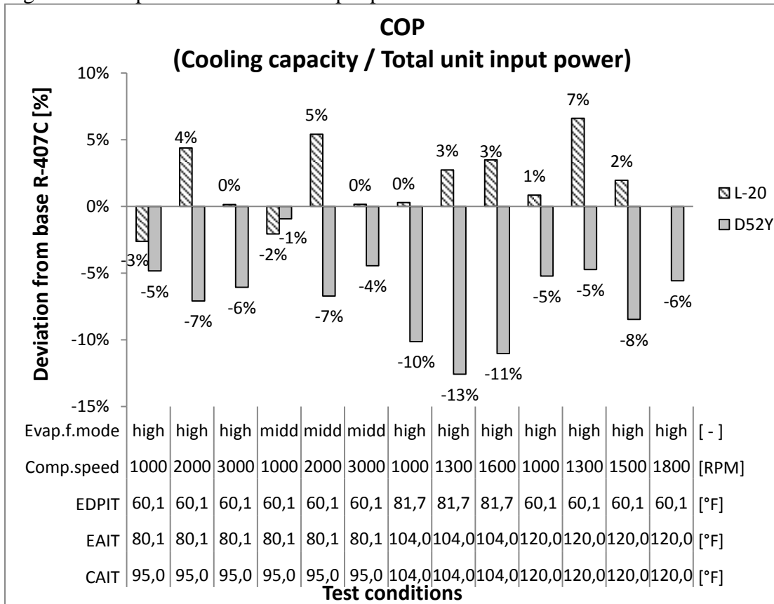
Figure 5: Comparison of COP relative to R-407C.
