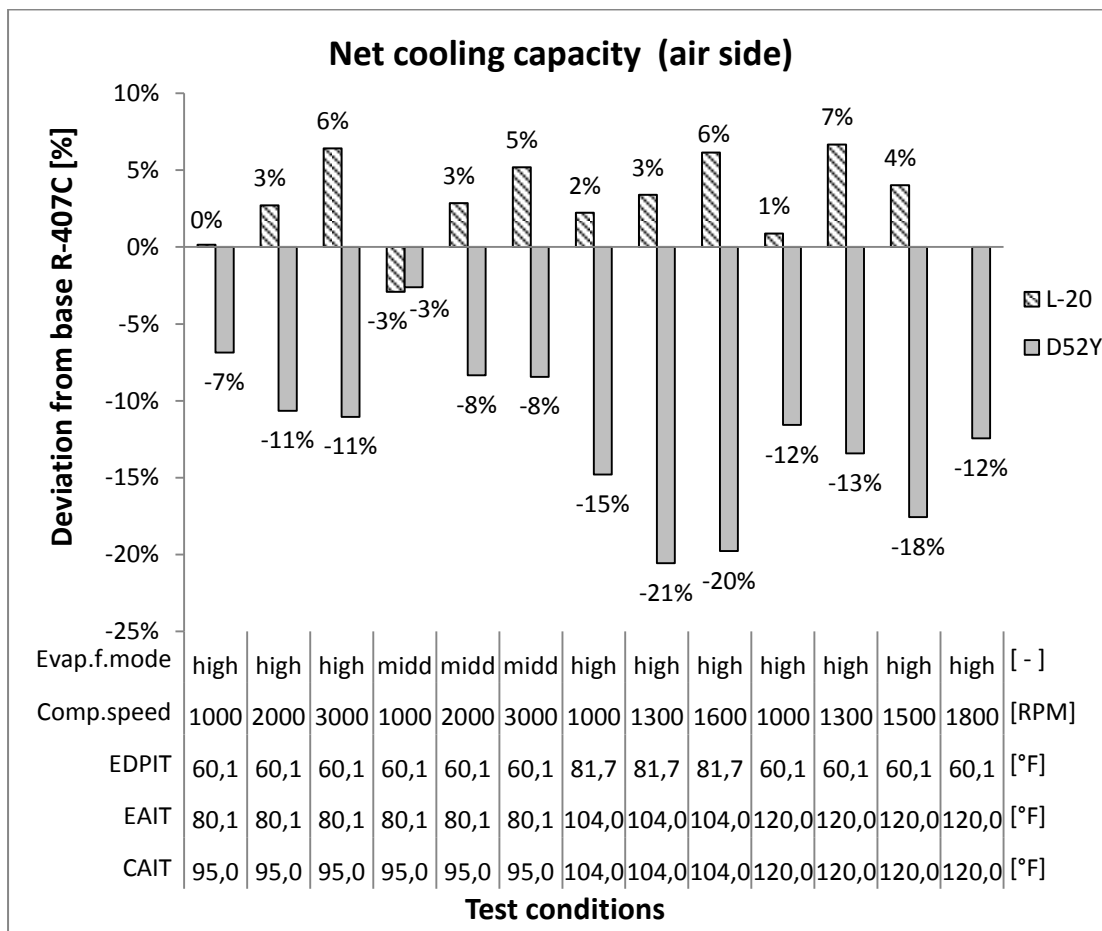
Figure 3: Comparison of net cooling capacity (air side) relative to R-407C.
