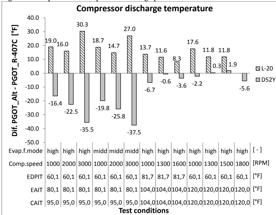
Figure 7: Comparison of compressor discharge temperature relative to R-407C.
