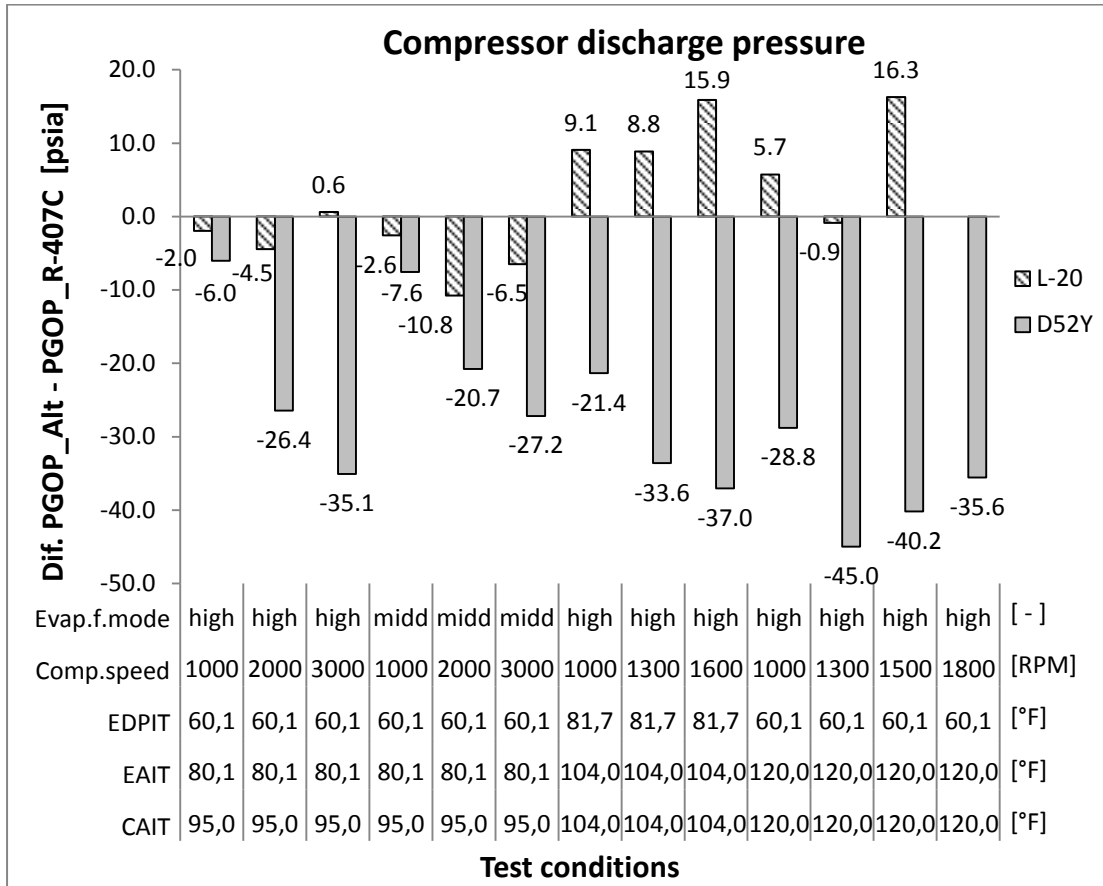
Figure 6: Comparison of compressor discharge pressure relative to R-407C.
