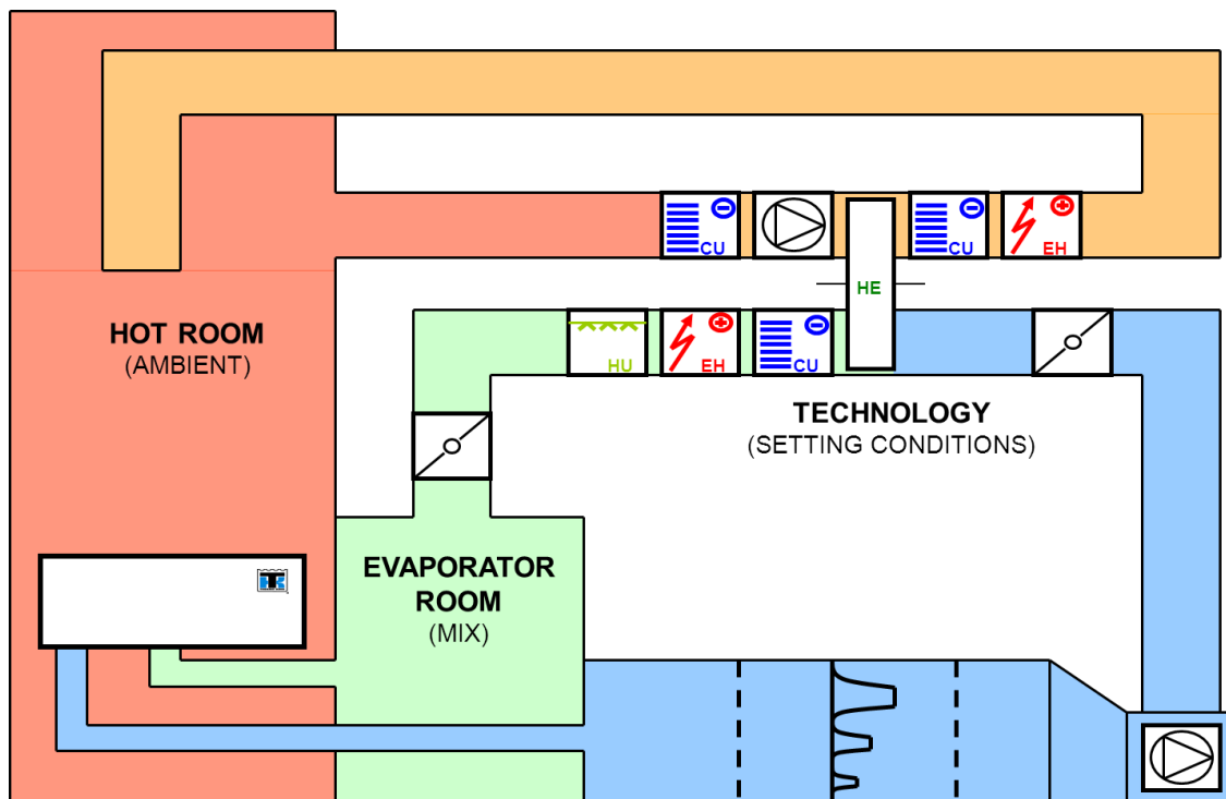
Figure 1: HVAC test lab design
