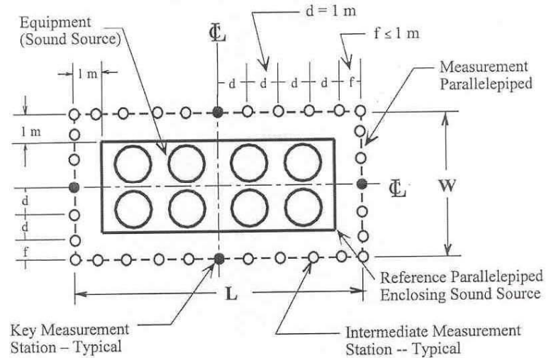
Figure D1. Plan View of Measurement Parallelepiped
