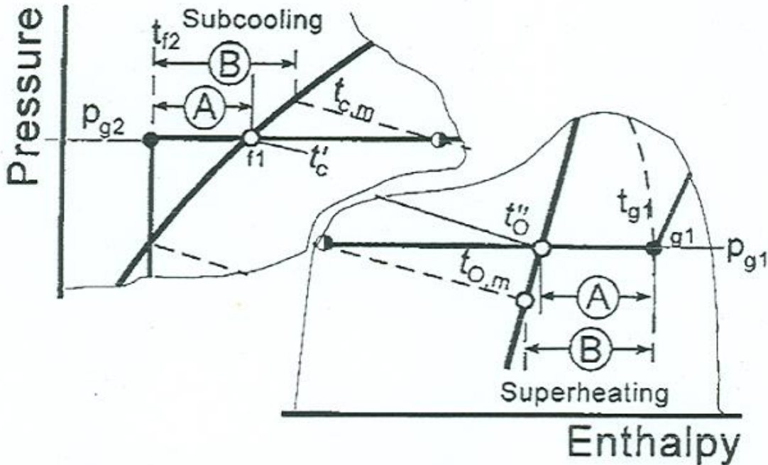
Figure C3. Definitions of Subcooling and Superheating
