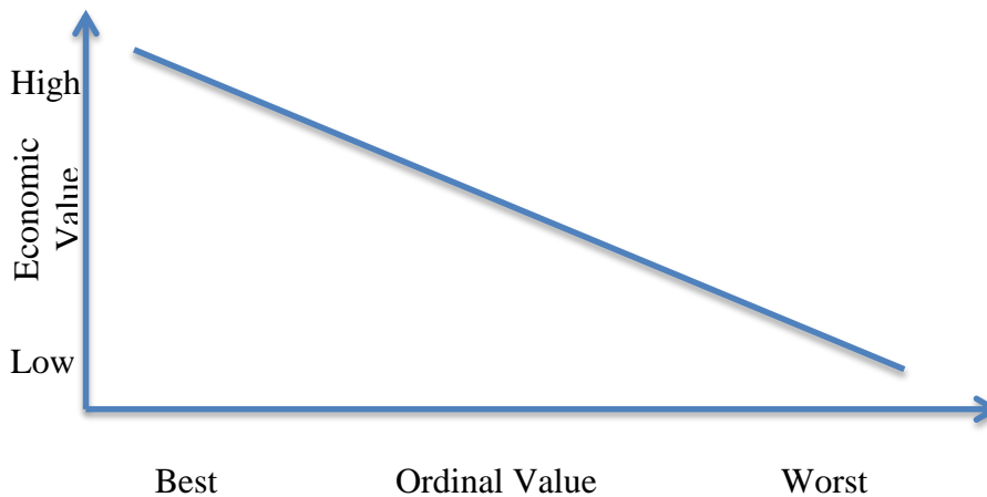
Figure 1: Ordinal Ranking
