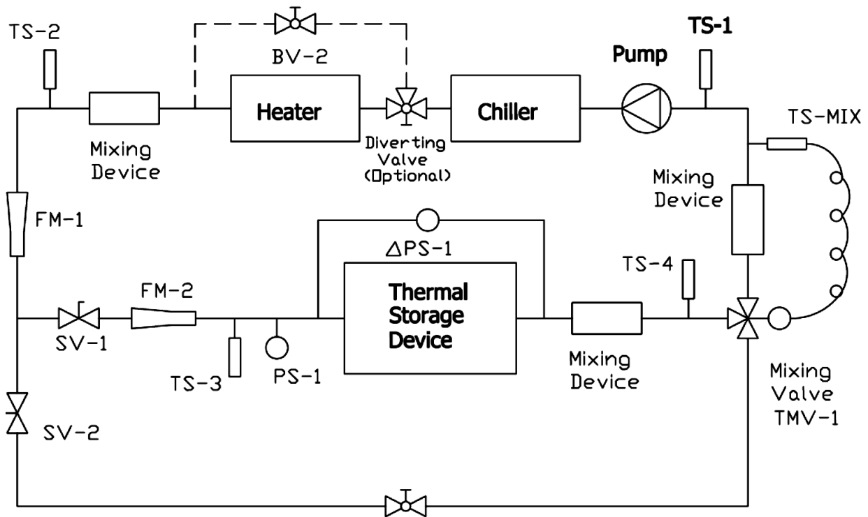
Figure C1. Thermal Storage Device Test Apparatus
