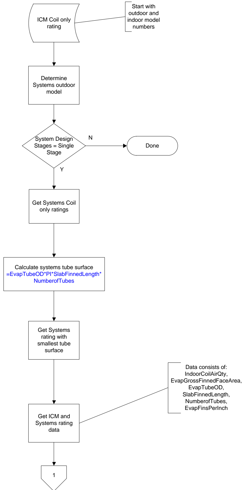
Figure G1: Part 1 of the ORNL Flowchart
