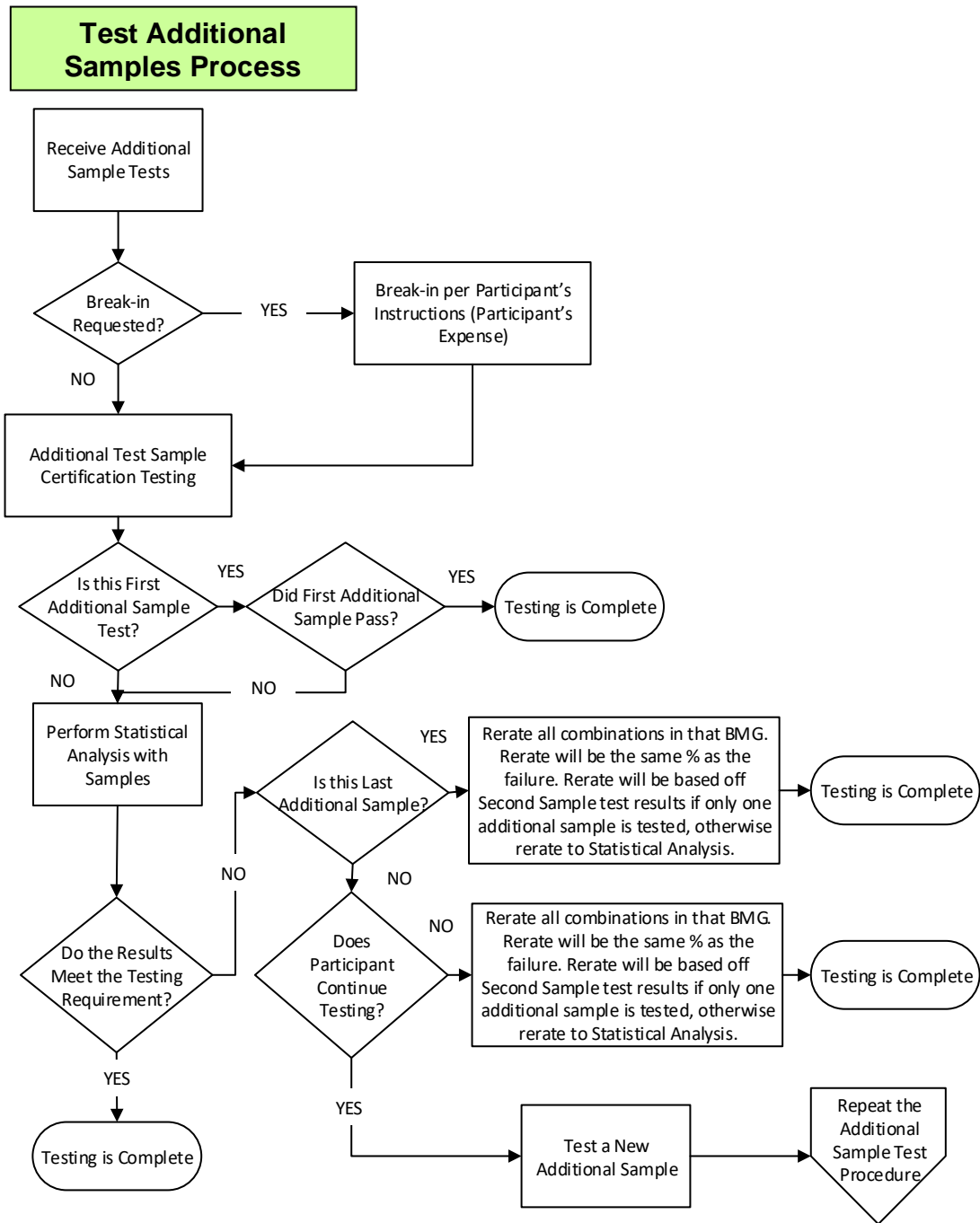
Figure D5: Test Additional Samples Process
