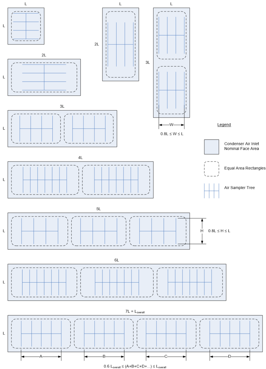
Figure 3 Example Determination of Measurement Rectangles and Required Number of Air Sampling Trees (Informative)
