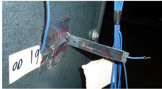
Figure C11. Typical Thermocouple Temperature Measuring Device Mounting
